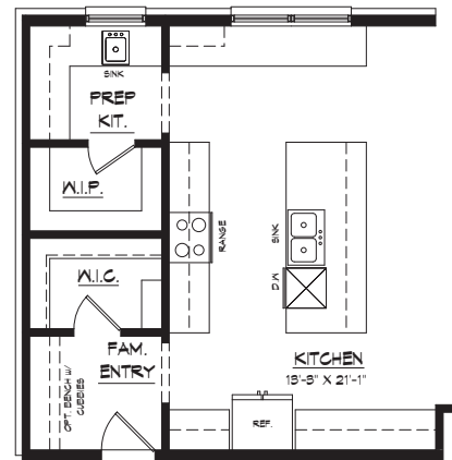
OPT. PREP KITCHEN FIRST FLOOR PLAN
