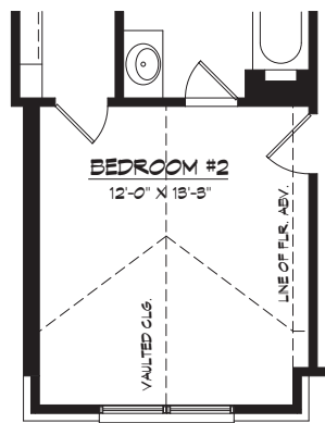
OPT. VAULTED CLG. SECOND FLOOR PLAN
