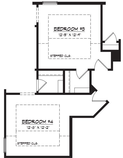
OPT. STEPPED CLGS. SECOND FLOOR PLAN
