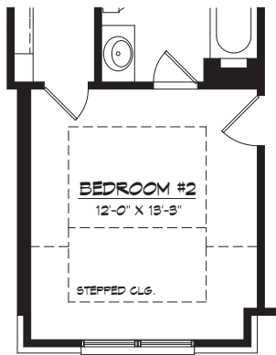
OPT. STEPPED CLG SECOND FLOOR PLAN
