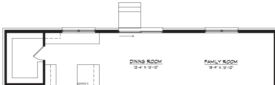
OPT. 3080 SLIDING GLASS DR. FIRST FLOOR PLAN
