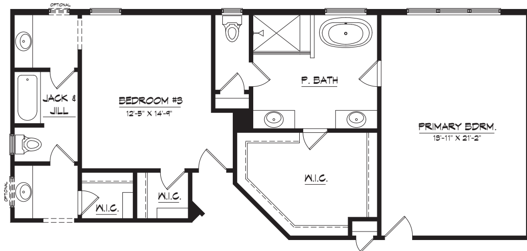
OPT. 2' EXTENSION SECOND FLOOR PLAN
