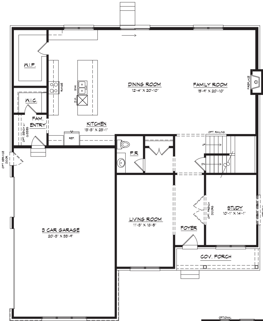
OPT. ALT. 4' EXTENSION FIRST FLOOR PLAN
