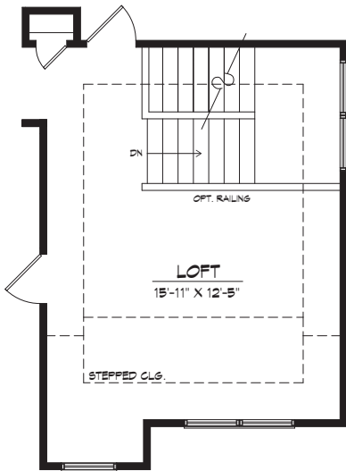
OPT. STEPPED CLG SECOND FLOOR PLAN
