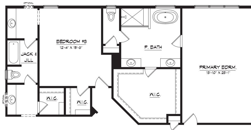
OPT. 4' EXTENSION SECOND FLOOR PLAN
