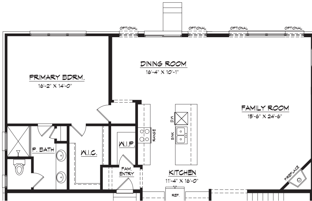
OPT. FAMILY EXTENSION FIRST FLOOR PLAN
