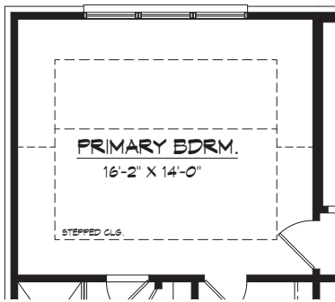
OPT. STEPPED CLG FIRST FLOOR PLAN
