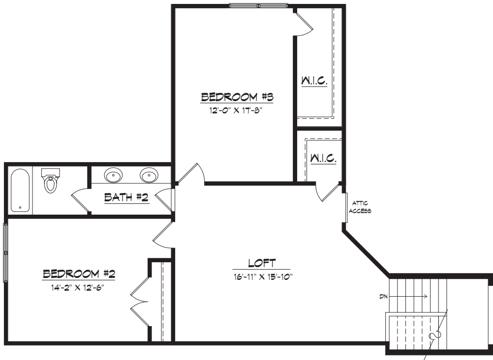
OPT. 2' EXTENSION SECOND FLOOR PLAN
