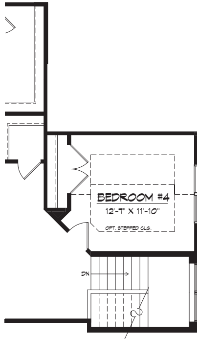
OPT. BEDROOM #4 SECOND FLOOR PLAN
