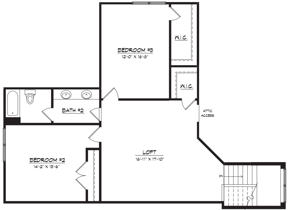
OPT. ALT. 4' EXTENSION SECOND FLOOR PLAN
