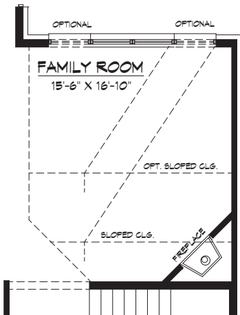
OPT. SLOPED CLG FIRST FLOOR PLAN
