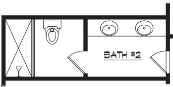
OPT. BATH #2 w/ ALT. 4' EXT. SECOND FLOOR PLAN
