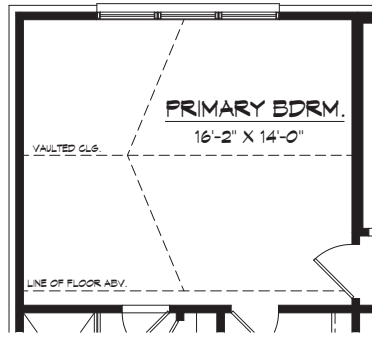
OPT. VAULTED CLG FIRST FLOOR PLAN
