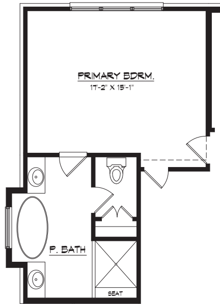
OPT. P. BATH FIRST FLOOR PLAN
