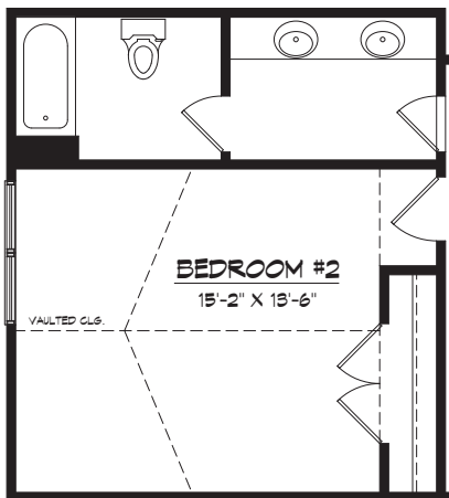
OPT. VAULTED CLG SECOND FLOOR PLAN
