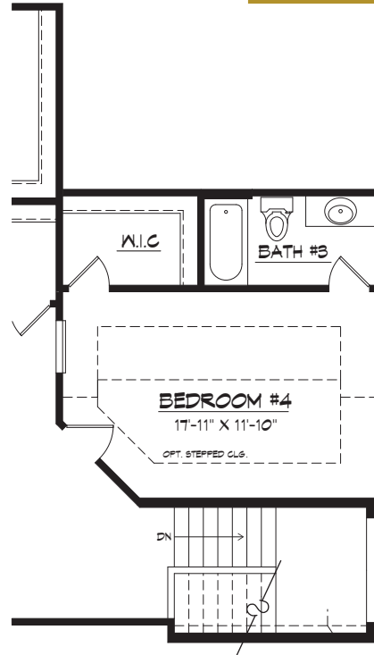
OPT. BEDROOM #4 W/ BATH SECOND FLOOR PLAN
