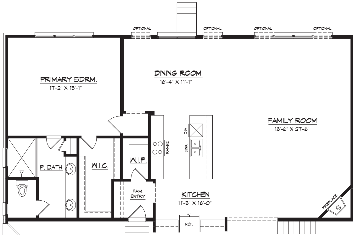
OPT. FAMILY EXTENSION FIRST FLOOR PLAN
